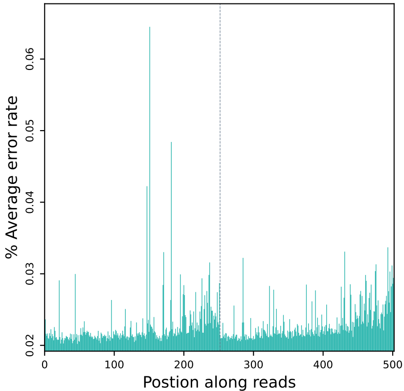
Error rate distribution along reads (R10715)
